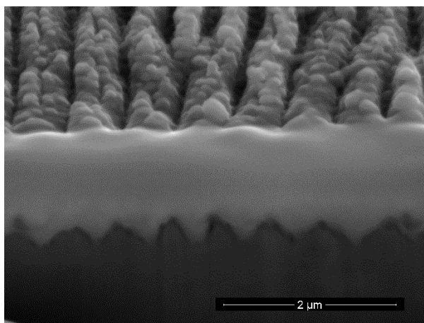
Fig. 3. FIB section of a sample processed at 0.8 mm/s. Structures with different profiles can be seen.
