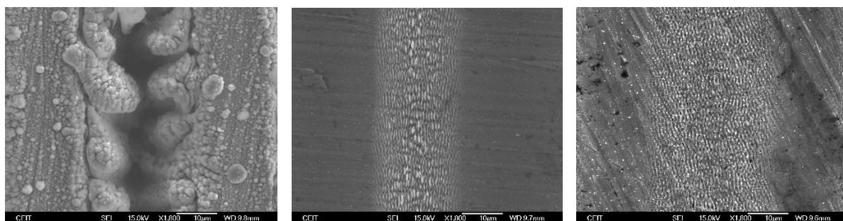
Fig.2. Different morphologies obtained depending on the number of pulses: ablation (left), LIPSS (middle) and nanobubbles (right).
