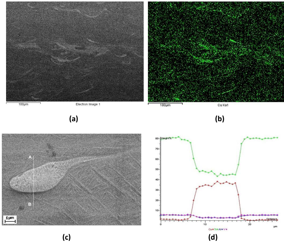
Fig. 5. Copper distribution map by XRD spectra (a) electron image, (b) Cu EDS map illustration of typical microstructures, (c), Cu-rich area and (d) elemental concentration profiles of Ti, Al, V and Cu in the Cu-rich area in wt.%, data obtained along line AB in (c).
