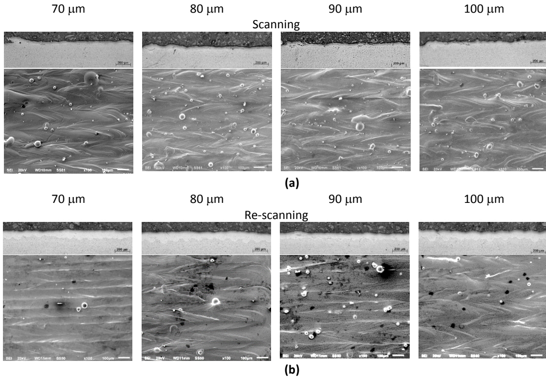
Fig. 1. Cross-sections and top view of DMLS surfaces from mixture Ti6Al4V (ELI) and 1 at.% Cu powders at laser power 170 W, scanning speed 1.0 m/s and 70–100 \mu\text{m} hatch distances: (a) single scan, (b) after rescanning.
